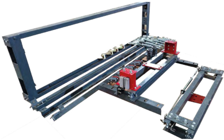
MR 1:1 CAR FRAME
